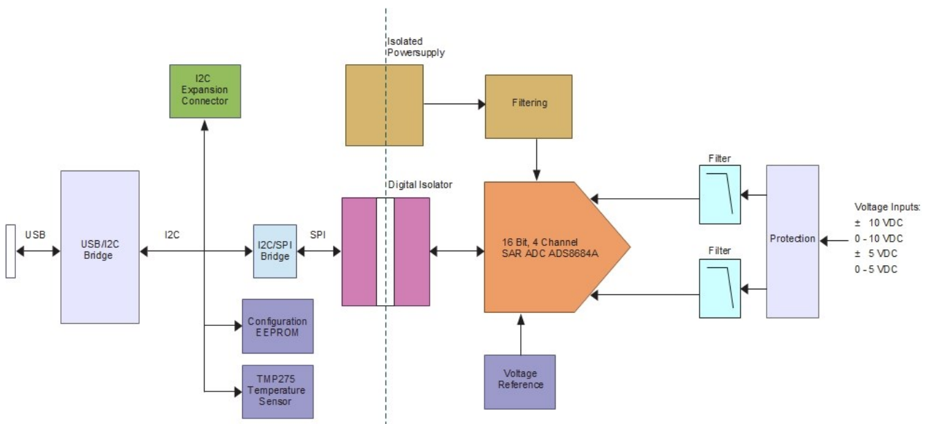
Fig. 1 Block Diagram
