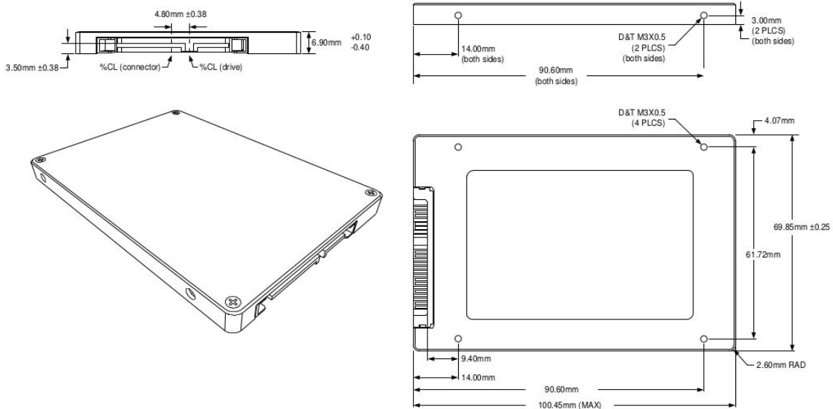
Figure 2-1. 250SH 2.5'' SSD Dimensions (7mm, 2TB)
