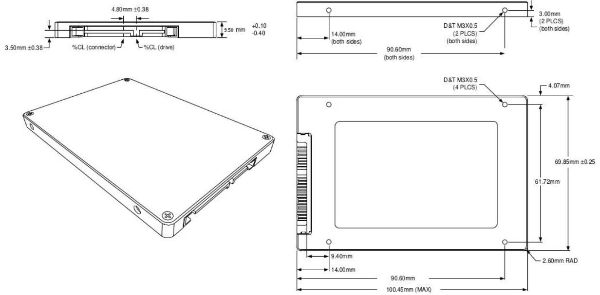
Figure 2-2. 250SH 2.5" SSD Dimensions (9.5mm, 4TB & 8TB std. Temp.)
