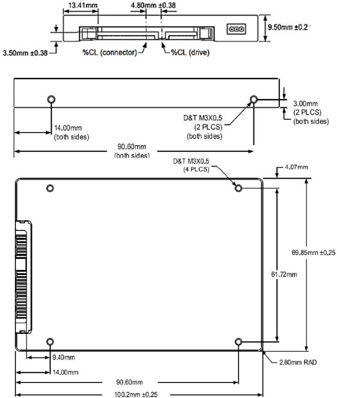
Figure 2-3. 250SH 2.5" SSD w/ jumper option Dimensions (9.5mm, 4TB & 8TB ext. temp.)
