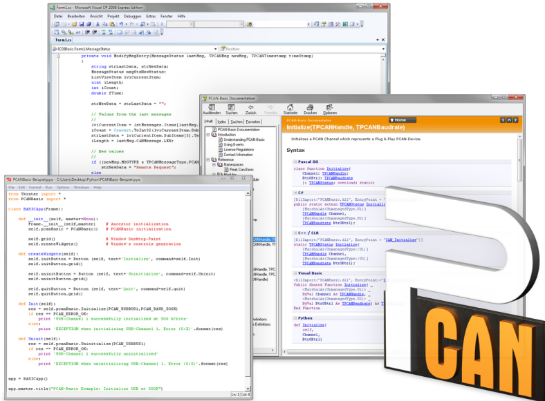
Figure 12: PCAN-Basic
